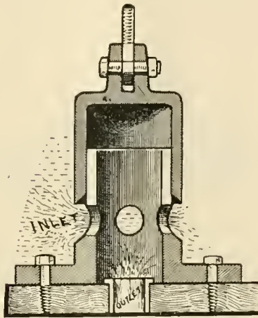
COTTER'S TENDER VALVE.
